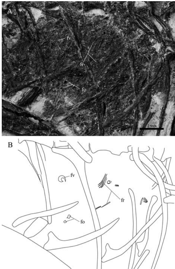
Figure 6. Detail photograph (A) and line drawing (B) of the food remains preserved in the abdominal cavity of Piscivoravis lii gen. et sp. nov. IVPP V17078. Abbreviations: fv, fish vertebra; fr, fin rays; fo, fish opercular fragments. Scale bar equals 5 mm (planned for single column width).
