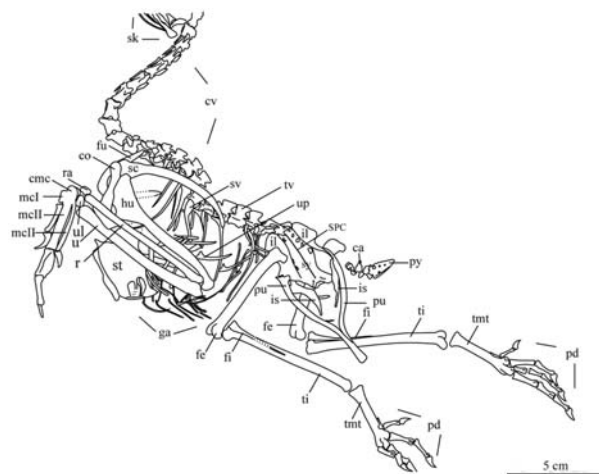
Figure 3. Line drawing of the holotype of Piscivoravis lii gen. et sp. nov. (IVPP V 17078). Abbreviations: al, alula; ca, caudal vertebra; cmc, carpometacarpus; co, coracoid; cv, cervical vertebra; fe, femur; fi, fibula; fu, furcula; ga, gastralia; hu, humerus; il, ilium; is, ischium; md, manual digits; mcl, alular metacarpal; mcII, major metacarpal; mcIII, minor metacarpal; mt, metatarsus; pd, pedal digits; pm, primaries; pu, pubis; py, pygostyle; r, radius; ra, radiale; sc, scapula; se, semilunate carpal; sk, skull; spc, spinal crest; sr, sternal rib; st, sternum; sy, synsacrum; ti, tibia; tmt, tarsometatarsus; tr, thoracic rib; u, ulna; ul, ulnare. Scale bar equals 1 cm (planned for single column width).
