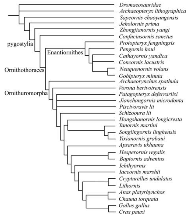
Figure 7. Strict consensus cladogram of the six MPTs (length 571) illustrating the hypothetical phylogenetic position of Piscivoravis lii gen. et sp. nov. CI: 0.4694, RI: 0.7432 (planned for single column width).
