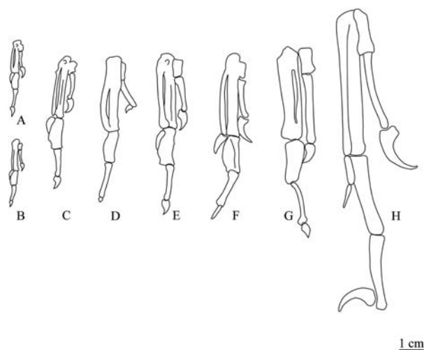
Figure 9. Comparison of the manus of Piscivoravis lii (F) with the other Early Cretaceous ornithuromorphs and Sapeornis chaoyangensis . A, Longicrusavis houi ; B, Hongshanornis longicresta ; C, Yanornis martini ; D, Schizooura lii ; E, Yixianornis grabaui ; G, Jianchang microdonta ; H, Sapeornis chaoyangensis [modified from Zhou and Zhang (2003) and O’Connor et al. (2010)]. Scale bar equals 1 cm (planned for single column width).
