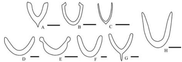
Figure 5. Comparison of the furcula of Piscivoravis lii (H) and the other Early Cretaceous ornithuromorphs. A, Schizoura lii ; B, Archaeorhynchus spathula ; C, Hongshanornis longicresta ; D, Archaeopteryx lithographica ; E, Confuciusornis sanctus ; F, Jeholornis prima ; G, Pengornis houii . Scale bar equals 10 mm. Modified from Zhou et al. (2012) (planned for single column width).
