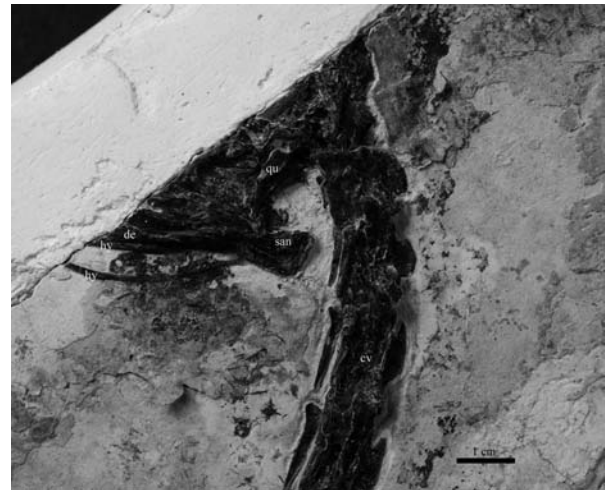
Figure 4. Photo of the skull of the holotype of Piscivoravis lii gen. et sp. nov. (IVPP V 17078). Abbreviations: an, angular; cv, cervical vertebra; de, dentary; hy, hyoid bone; qu, quadrate; san, surangular. Scale bar equals 1 cm (planned for single column width).
