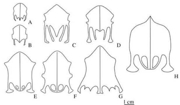
Figure 8. Comparison of the sternum of Early Cretaceous ornithuromorphs. A, Hongshanornis longicresta ; B, Longicrusavis hou ; C, FRDC – 05 – CM – 02; D, Archaeorhynchus spathula ; E, Yixianornis grabau ; F, Yanornis martini ; G, Jianchangornis microdonta ; H, Piscivoravis lii . Modified from Zhou et al. (2013). Scale bar equals 1 cm (planned for single column width).
